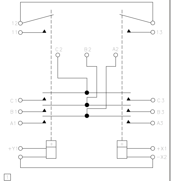
TERMINAL TYPE 3
