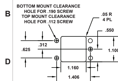
Recommended Mounting Panel Cutout
