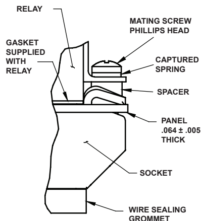
Mounting Hardware
